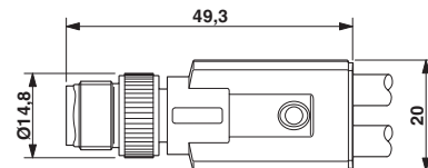
Dimensioned drawing
