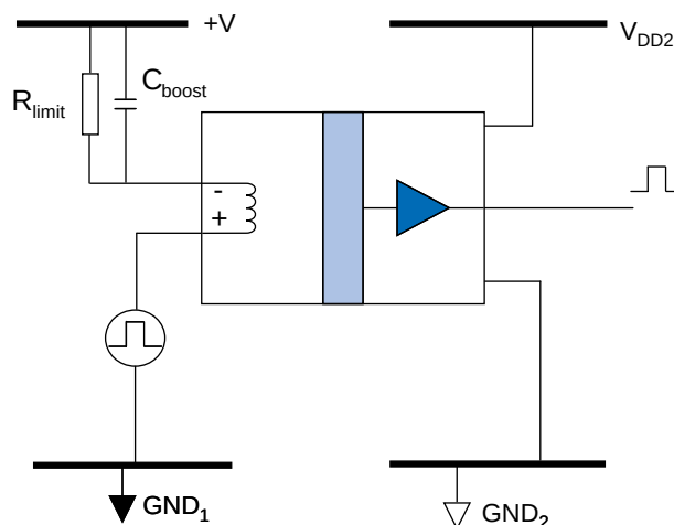
Non-inverting Configuration
