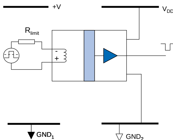
Differential Configuration
