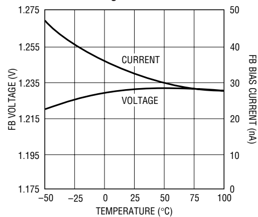
FB Pin Voltage and Bias Current
