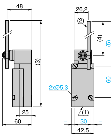
XCKJ110559
