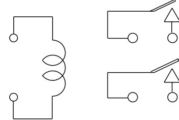
CONNECTION DIAGRAM (BOTTM VIEW) 接続図
