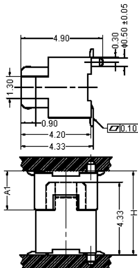
Mating Draw (Reference)
