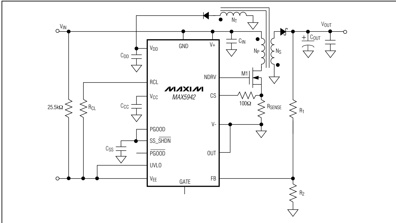
Figure 6. Flyback Converter
