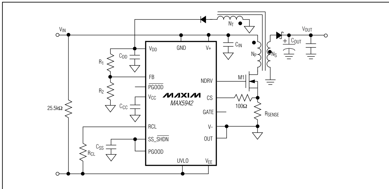
Figure 7. Flyback Converter
