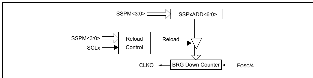
FIGURE 16-17: BAUD RATE GENERATOR BLOCK DIAGRAM
