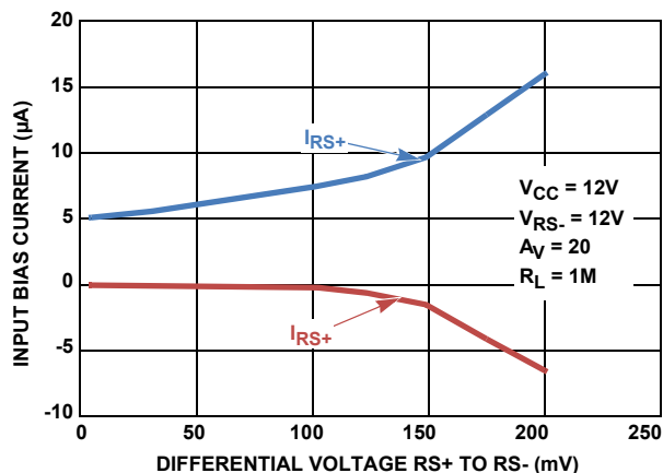
FIGURE 70. HIGH SIDE CURRENT SENSING INPUT BIAS CURRENTS
