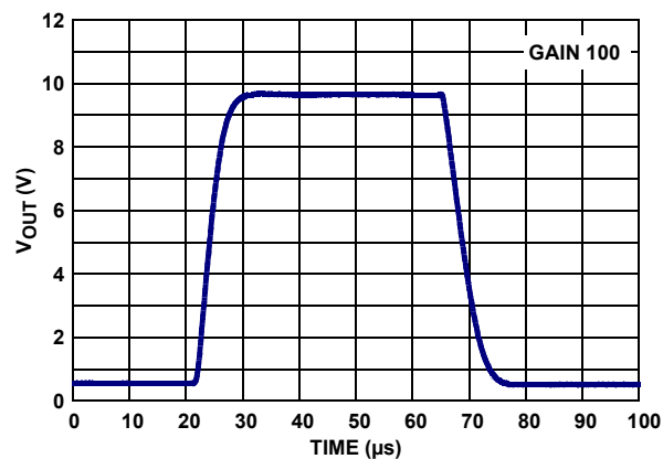
FIGURE 6. LARGE SIGNAL TRANSIENT RESPONSE V_{RS+} = 12V , V_{SENSE} = 100mV
