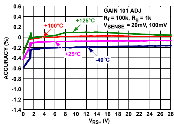
FIGURE 60. GAIN ACCURACY vs V_{RS+} = 0V TO 28V
