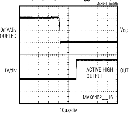
PROPAGATION DELAY V_{CC} FALLING
