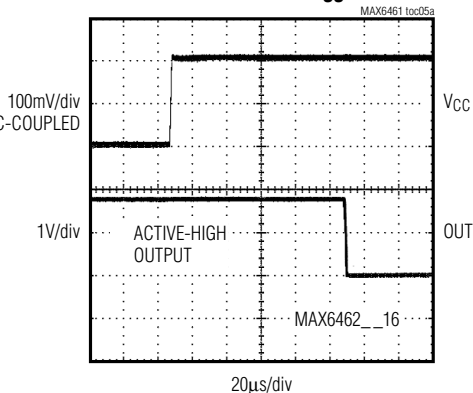
PROPAGATION DELAY V_{CC} RISING
