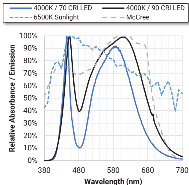
Spectral Power Distribution (White)
