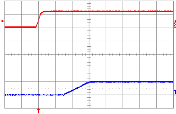
Fig. 1.0V.5: Turn-on transient for V_{out} = 1.0 V with application of V_{in} at full rated load current (resistive) and 47 \mu F external capacitance at V_{in} = 12 V. Top trace: V_{in} (10 V/div.); Bottom trace: output voltage (1 V/div.); Time scale: 5 ms/div.
