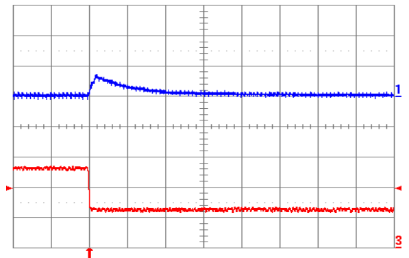
Fig. 1.0V.8: Output voltage response for V_{out} = 1.0 V to negative load current step change from 5 A to 2.5 A with slew rate of -5 A/ \mu s at V_{in} = 12 V. Top trace: output voltage (100 mV/div.); Bottom trace: load current (2 A/div.). C_o = 47 \mu F ceramic. Time scale: 20 \mu s/div.
