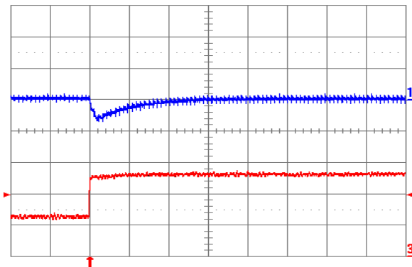
Fig. 1.0V.7: Output voltage response for V_{out} = 1.0 V to positive load current step change from 2.5 A to 5 A with slew rate of 5 A/ \mu s at V_{in} = 12 V. Top trace: output voltage (100 mV/div.); Bottom trace: load current (2 A/div.). C_o = 47 \mu F ceramic. Time scale: 20 \mu s/div.
