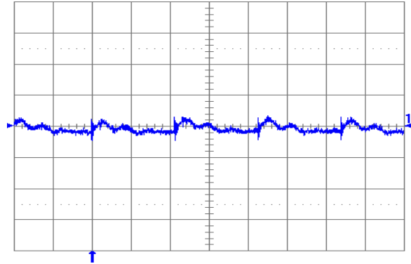
Fig. 1.0V.6: Output voltage ripple (20 mV/div.) at full rated load current into a resistive load with external capacitance 47 \mu F ceramic + 1 \mu F ceramic, and V_{in} = 12 V for V_{out} = 1.0 V. Time scale: 1 \mu s/div.
