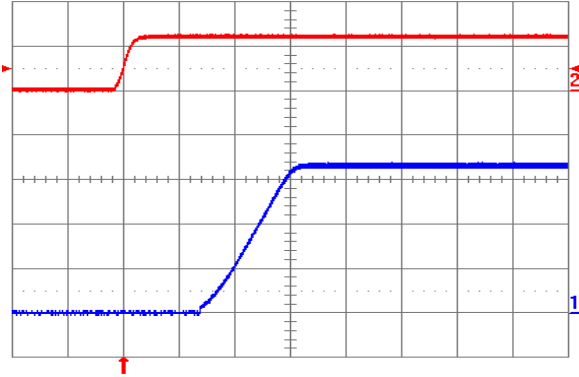
Fig. 3.3V.5: Turn-on transient for V_{out} = 3.3 V with application of V_{in} at full rated load current (resistive) and 47 \mu\text{F} external capacitance at V_{in} = 12 V. Top trace: V_{in} (10 V/div.); Bottom trace: output voltage (1 V/div.); Time scale: 5 ms/div.
