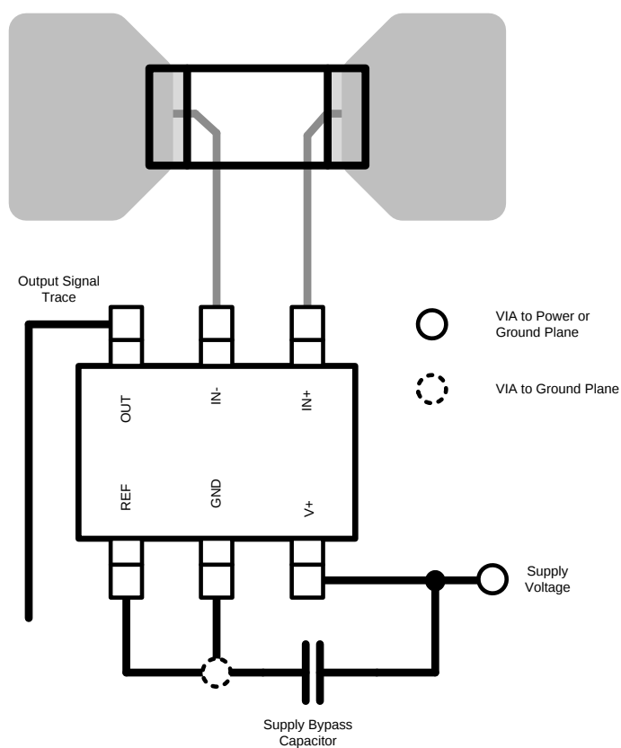
Figure 34. Recommended Layout
