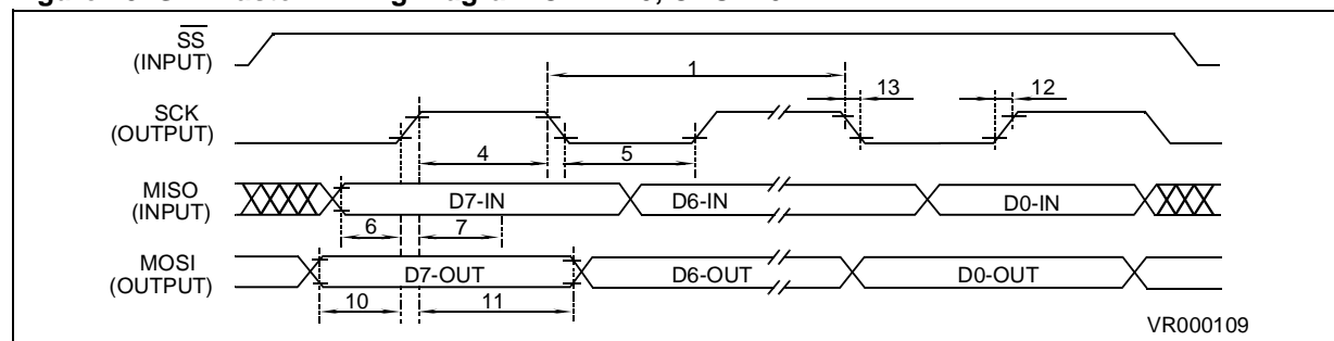
Figure 43. SPI Master Timing Diagram \text{CPHA}=0 , \text{CPOL}=0
