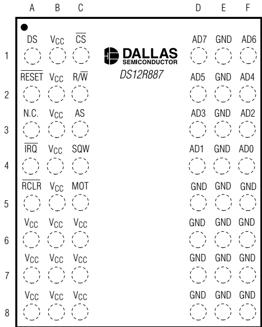
48 BGA
