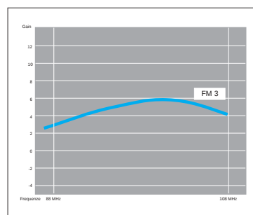
FM 3 elem.
