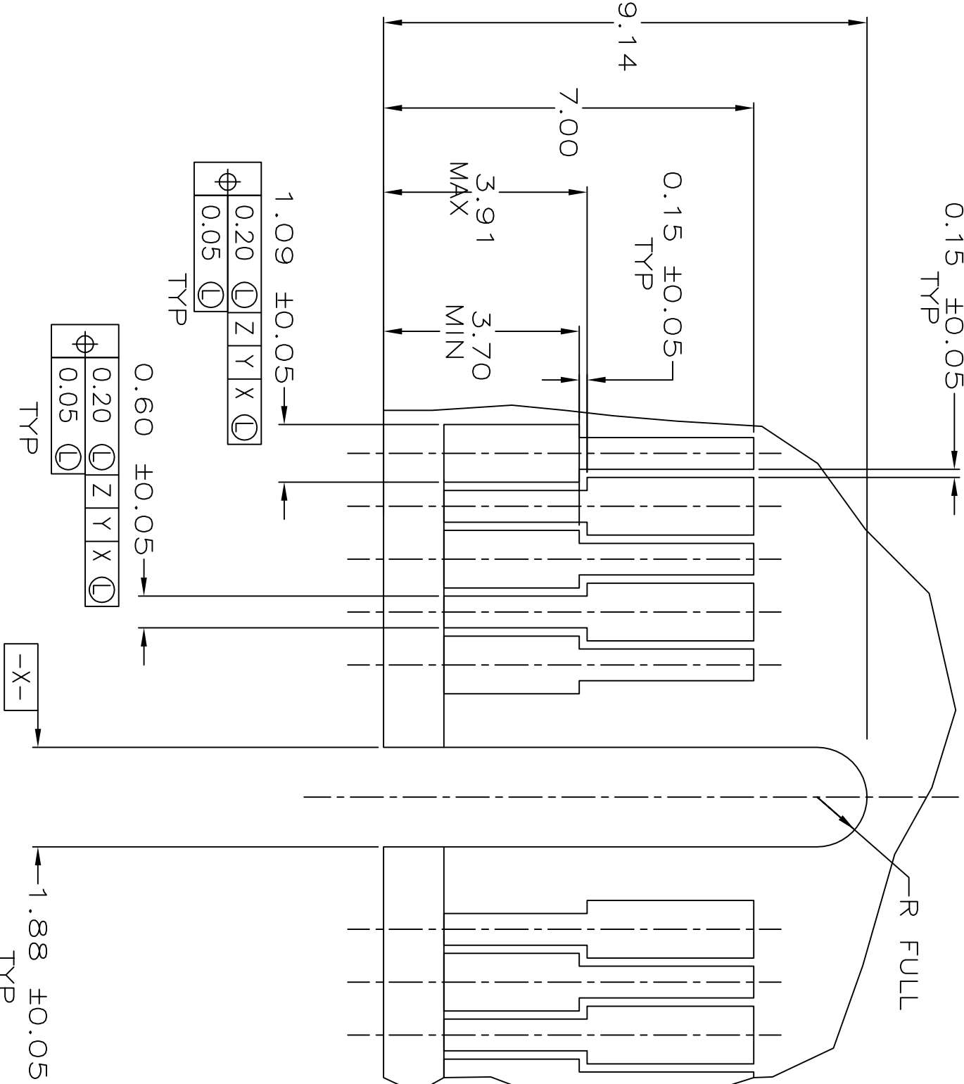
DETAIL D SCALE 10:1
