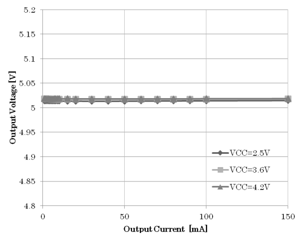
Figure 23. CH2 Output voltage vs Output Current
