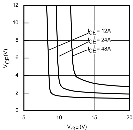
Fig. 12 - Typical V_{CE} vs. V_{GE} T_J = 175^\circ\text{C}
