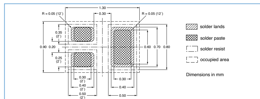
SOT883 (SC-101)
