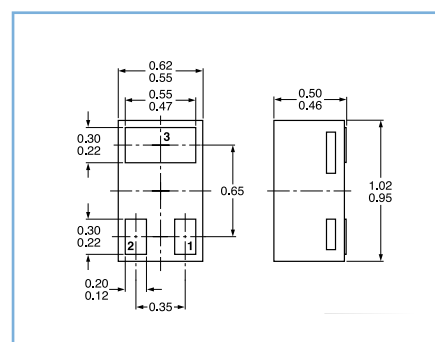
SOT883 (SC-101)
