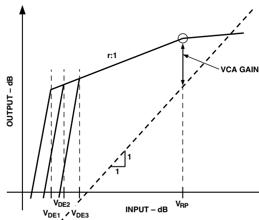
Figure 5. Effects of Varying the Downward Expansion (Noise Gate) Threshold
