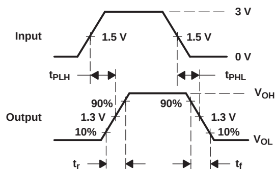
VOLTAGE WAVEFORMS
