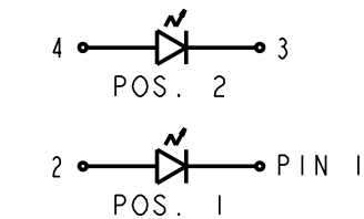
LEAD CONFIGURATION
