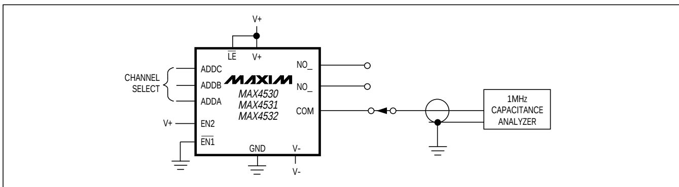
Figure 6. NO/COM Capacitance
