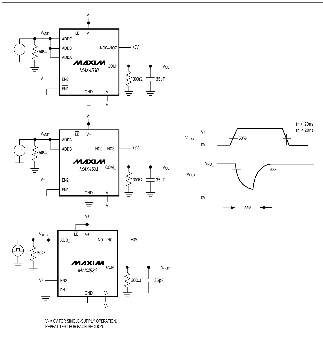
Figure 3. Break-Before-Make Interval
