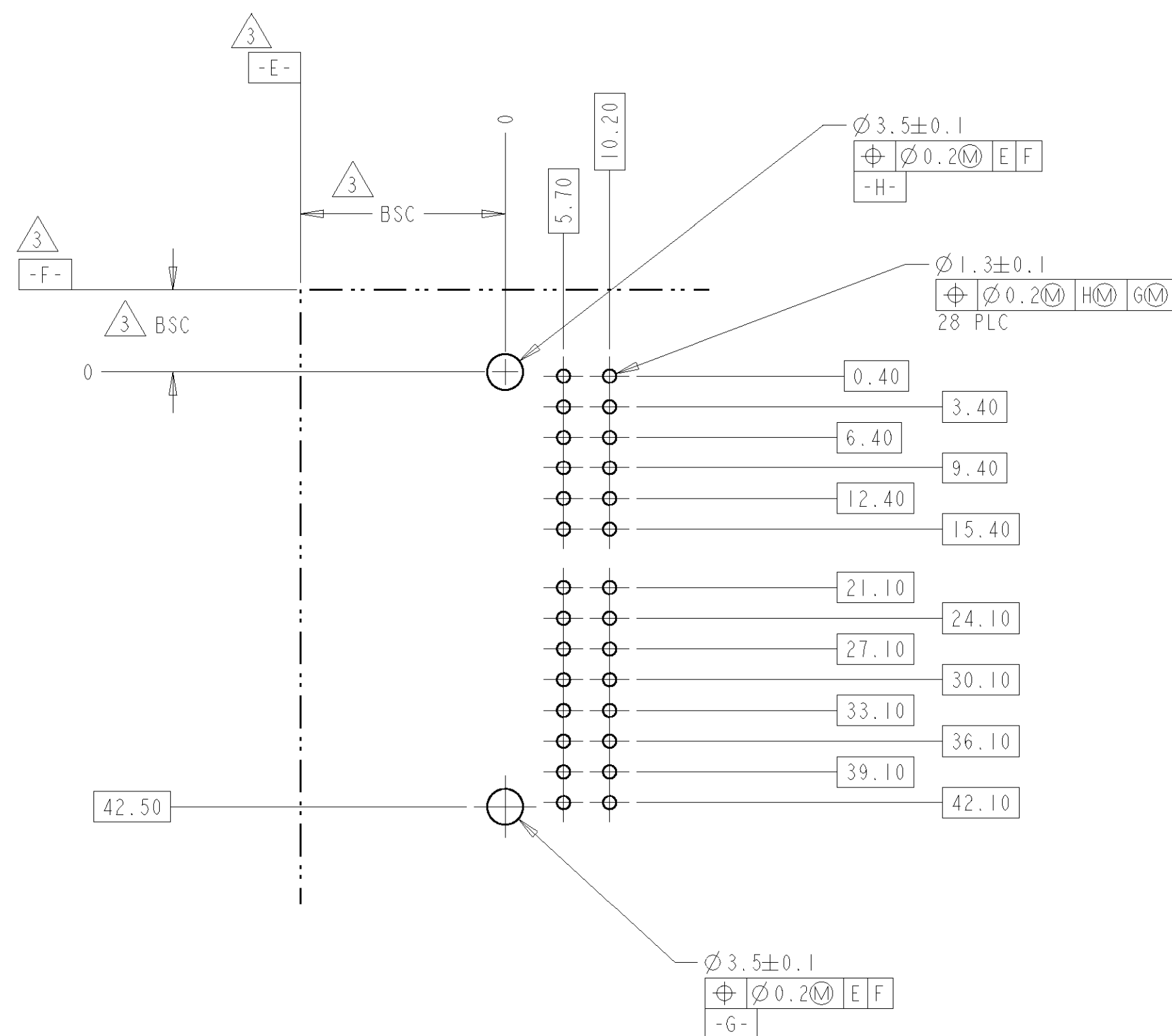
PC BOARD LAYOUT (SOLDER SIDE) (RECOMMENDED BOARD THICKNESS 1.57mm)
