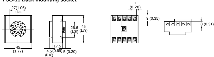
(Bottom view)
