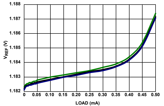
FIGURE 8. V_{REF} vs LOAD (SINK)
