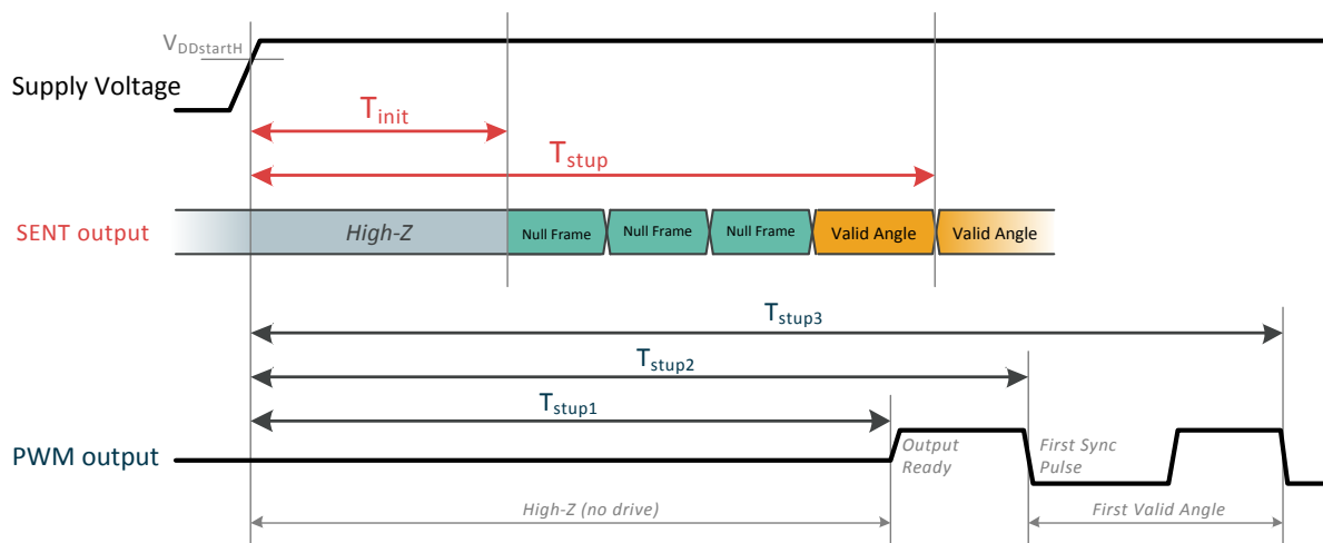
fig. 5 - Startup Time Definition
