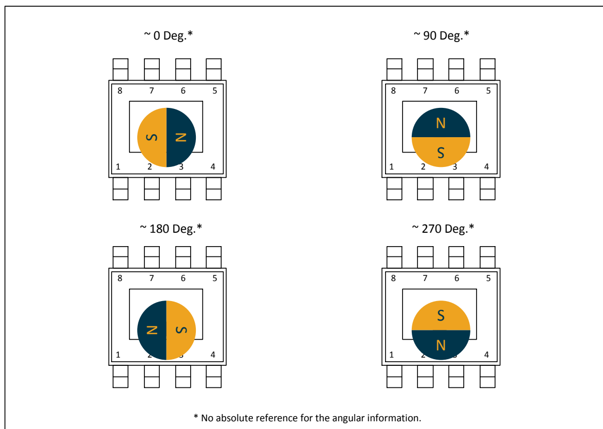
fig. 32 - SOIC-8 Angle Detection
