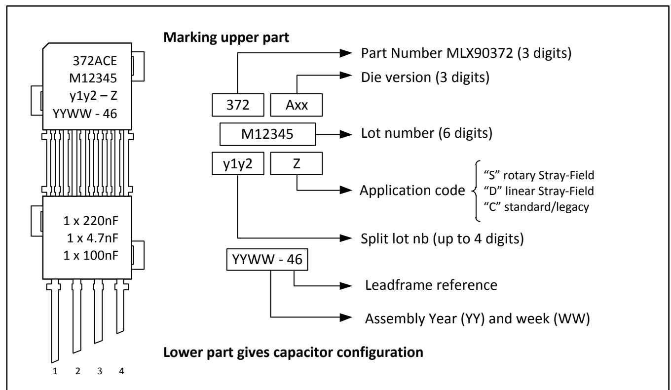
fig. 43 - DMP-4 Marking
