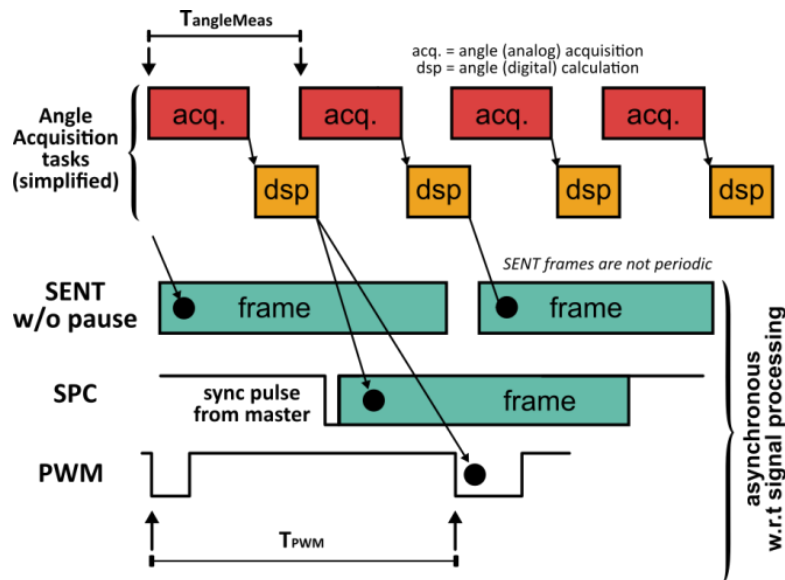
fig. 3 - Continuous Asynchronous Timing Mode
