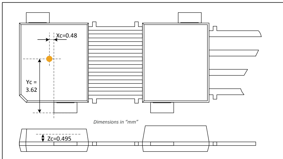
fig. 45 - DMP-4 Rotary Stray-field or legacy Sensitive Spot Position
