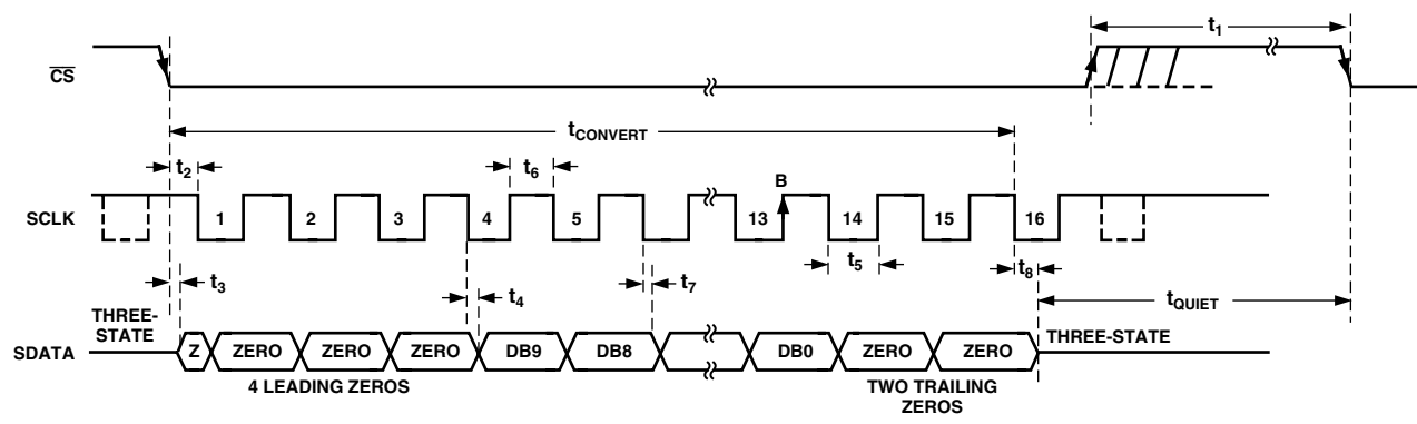
Figure 22. AD7477 Serial Interface Timing Diagram
