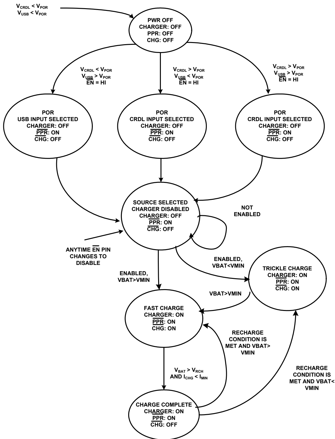
FIGURE 12. STATE DIAGRAM
