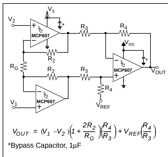
FIGURE 3-13: Three Op-Amp Instrumentation Amplifier
