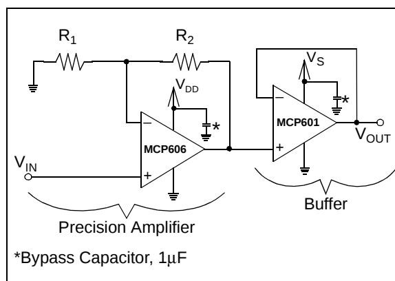
FIGURE 3-14: Precision Gain with Good Load Isolation
