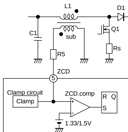
Fig.9 ZCD circuit
