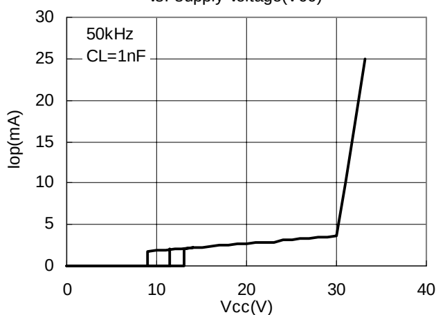
Dynamic operating power supply current( I_{OP} ) vs. supply voltage( V_{CC} )
