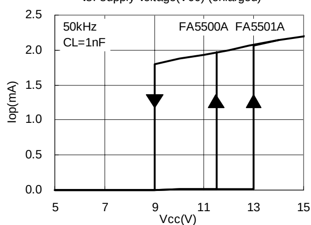
Dynamic operating power supply current( I_{OP} ) vs. supply voltage( V_{CC} ) (enlarged)
