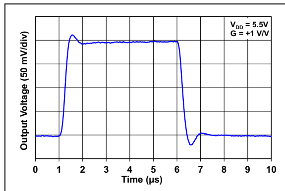
FIGURE 2-47: Non-Inverting Small Signal Step Response.
