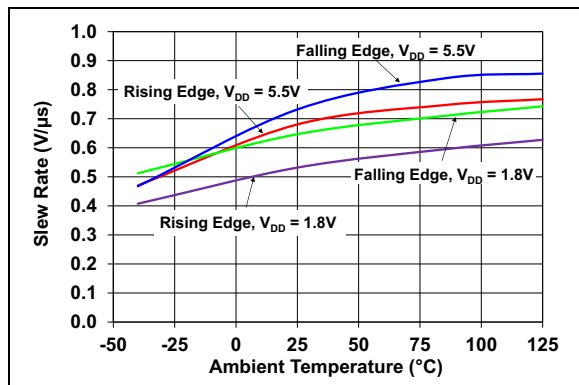
FIGURE 2-51: Slew Rate vs. Ambient Temperature.
