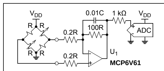
FIGURE 4-11: Simple Design.
