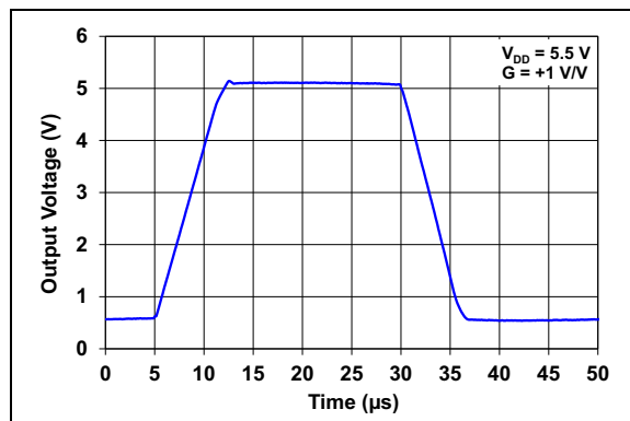
FIGURE 2-48: Non-Inverting Large Signal Step Response.
