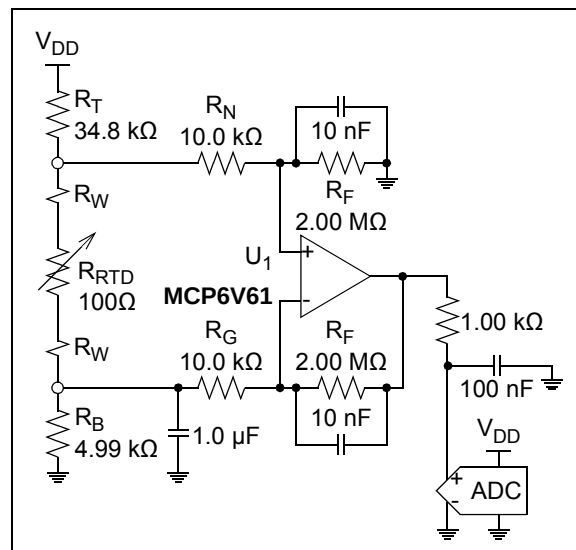
FIGURE 4-12: RTD Sensor.
