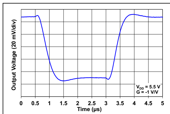
FIGURE 2-49: Inverting Small Signal Step Response.
