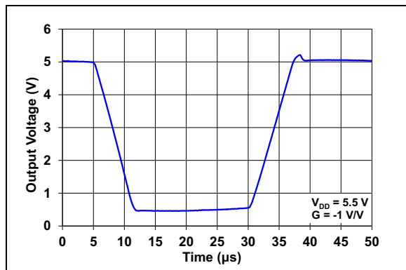
FIGURE 2-50: Inverting Large Signal Step Response.
