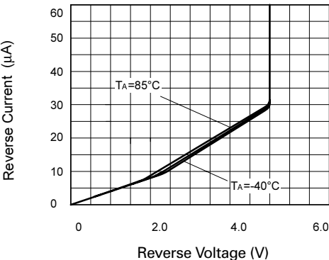
Reverse Characteristics
