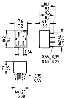
Package Dimensions mm
