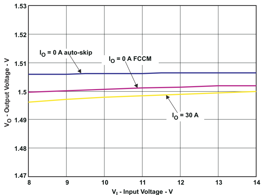
Figure 7-3. Line Regulation
