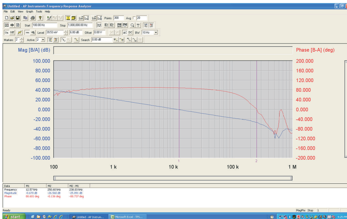
Figure 7-14. Bode Plot at 12 V IN , 1.5 V/30 A
