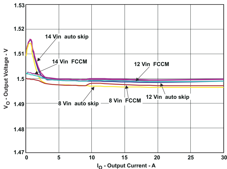
Figure 7-2. Load Regulation
