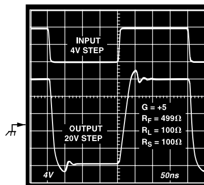
Figure 27. Driver 20 V Step Response, G = +5
