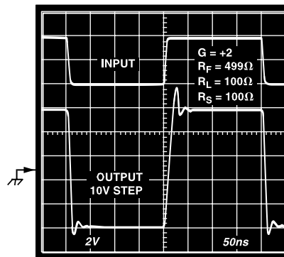
Figure 25. 10 V Step Response, G = +2
