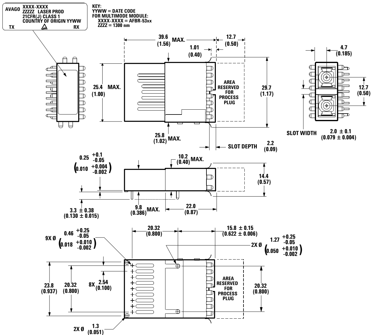
Figure 8. Package Outline for AFBR-53D3FZ.
