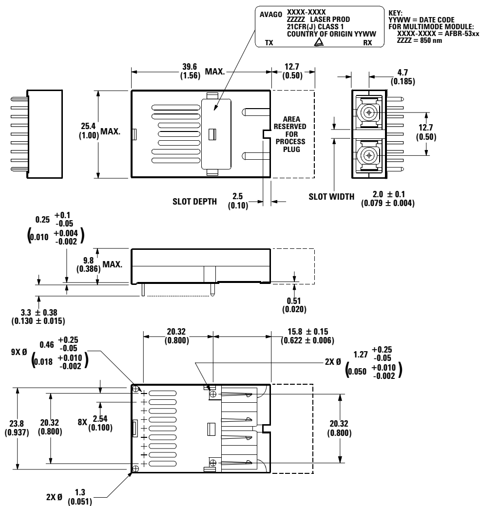
Figure 5. Package Outline Drawing for AFBR-53D3Z.
