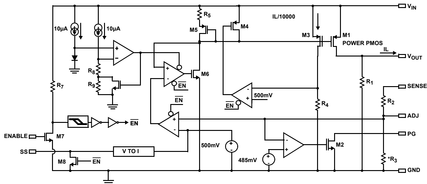
FIGURE 3. BLOCK DIAGRAM
