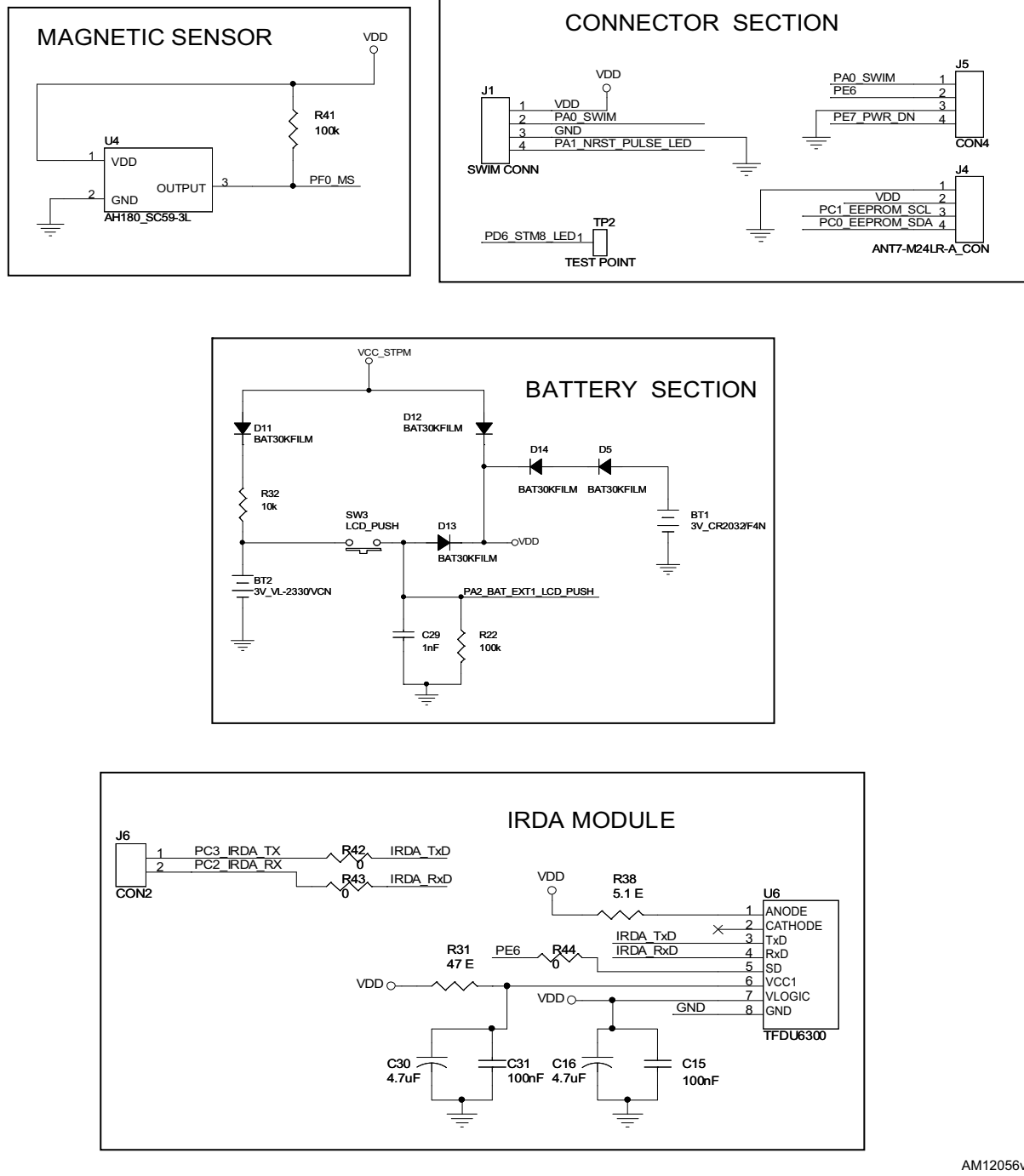
Figure 2. Schematic (2 of 4)
