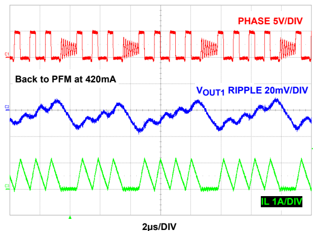
FIGURE 45. PWM TO PFM TRANSITION
