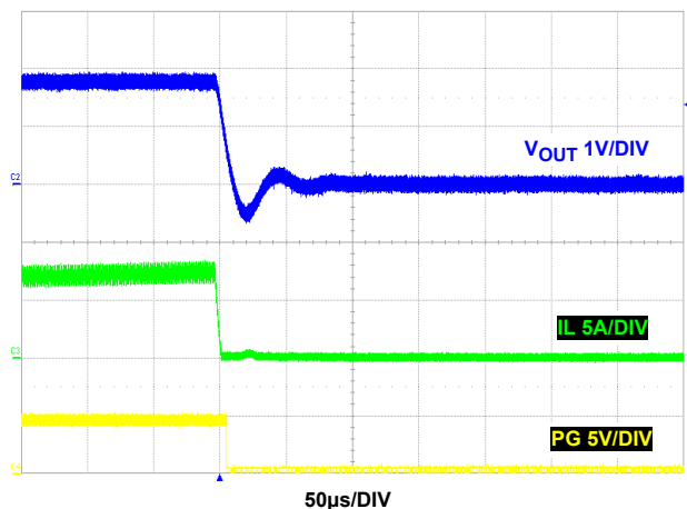
FIGURE 43. OVERCURRENT PROTECTION
