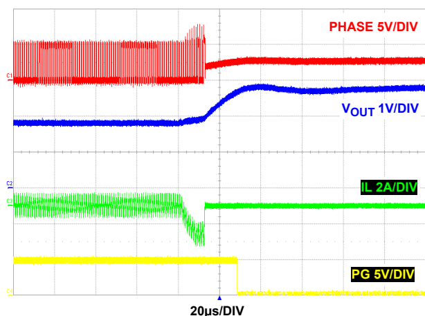
FIGURE 46. OVERVOLTAGE PROTECTION
