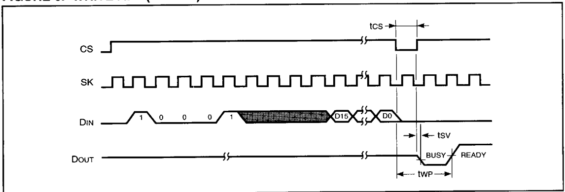
FIGURE 6. WRITE ALL (WRALL) TIMING
