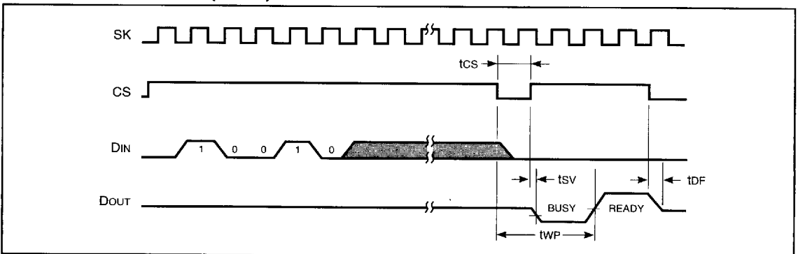
FIGURE 9. ERASE ALL (ERAL) CYCLE TIMING
