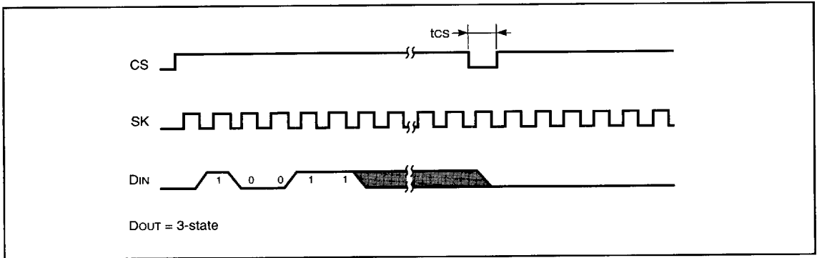
FIGURE 4. SYNCHRONOUS DATA TIMING
