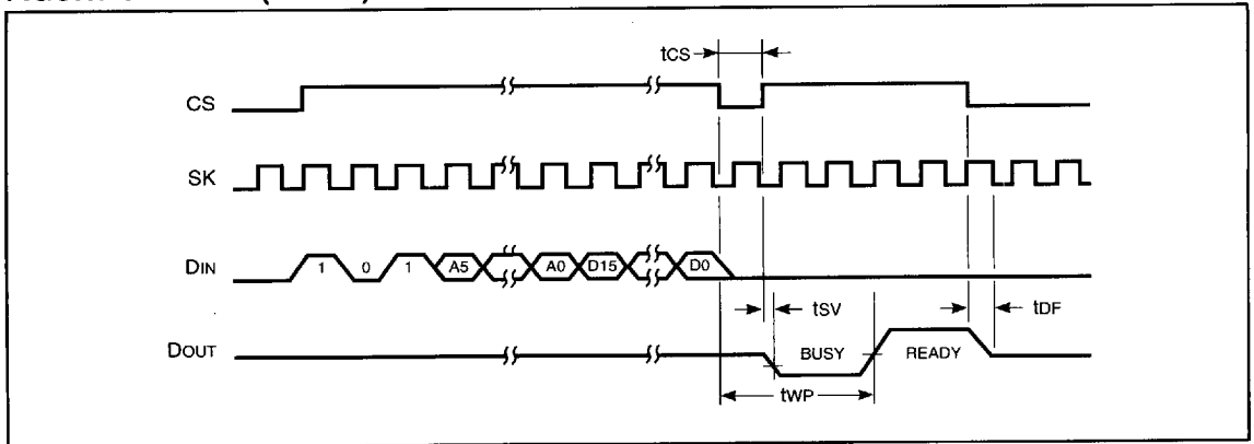
FIGURE 5. WRITE (WRITE) CYCLE TIMING
