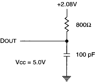
FIGURE 1. AC TEST CONDITIONS
