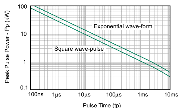
Figure 1. Non-repetitive peak pulse power rating curve
