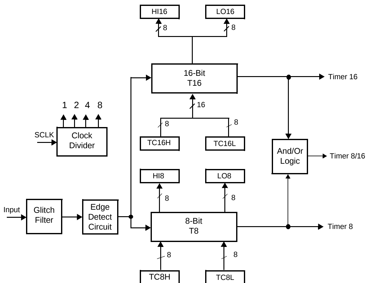
Figure 1. Counter/Timers Diagram
