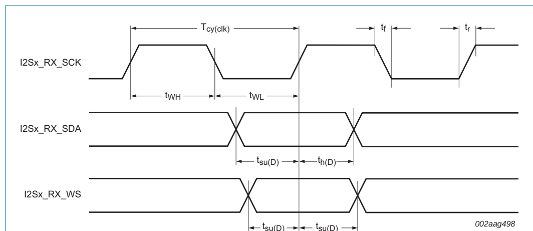
Fig 27. I 2 S-bus timing (receive)
