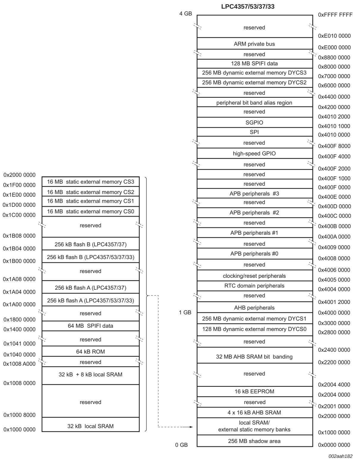
Fig 8. LPC4357/53/37/33 Memory mapping (overview)
