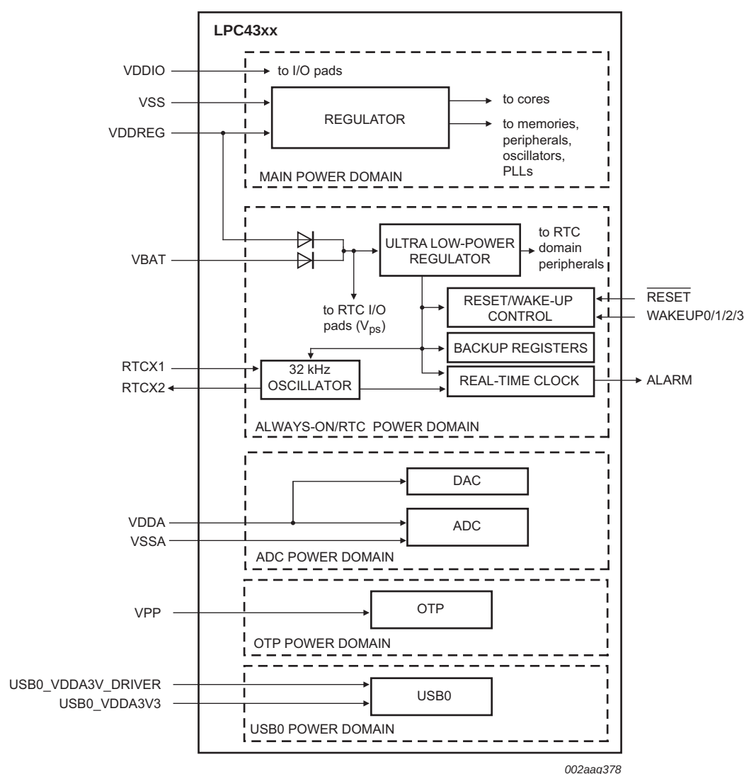
Fig 10. Power domains
