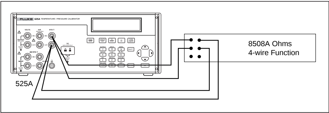
Figure 6-6. Connecting for Measuring Resistance Output
