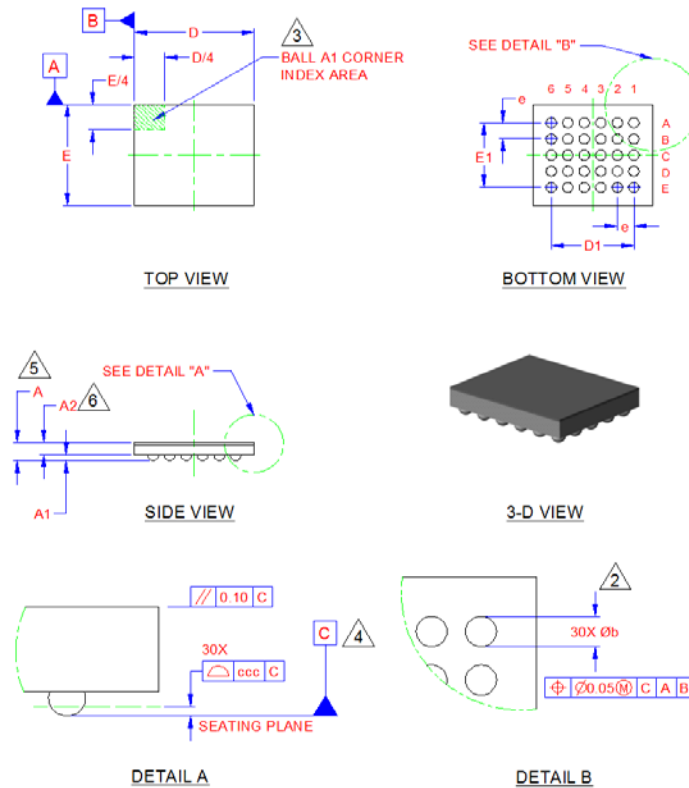
Figure 10.1 30-WLCSP Package
