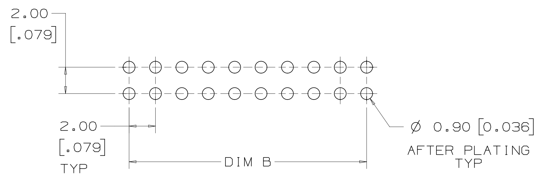
RECOMMENDED PCB HOLE PATTERN TOLERANCE = \pm 0.05 [ .002 ]
