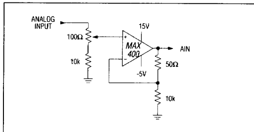
Figure 18. Adjusting Analog Input Gain to Trim Out Initial Reference Voltage Error
