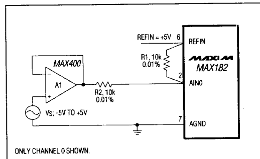
Figure 14. Bipolar -5V to +5V Operation
