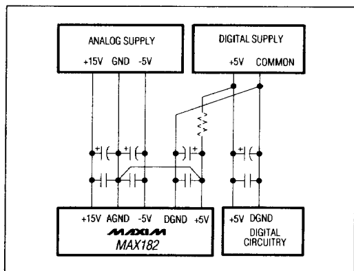
Figure 16. Power-Supply Grounding
