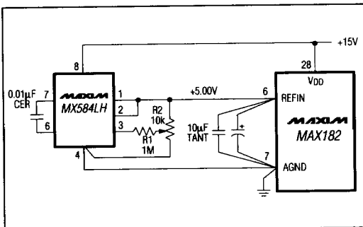
Figure 19. MX584LH as Reference Generator
