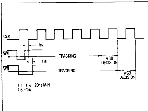
Figure 7. Width of Tracking Interval as a Function of WR Rising Edge Timing with Respect to CLK Falling Edge
