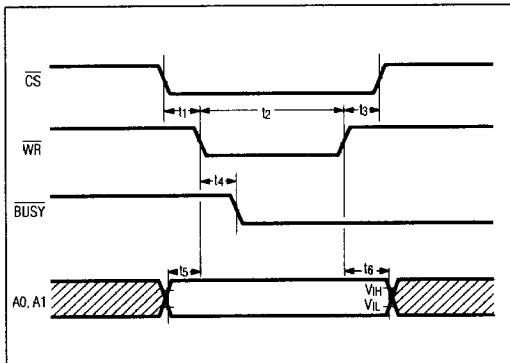
Figure 1: Start Cycle Timing
