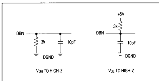
Figure 4. Load Circuits for Output Three-State Delay Test ( t_{14} )
