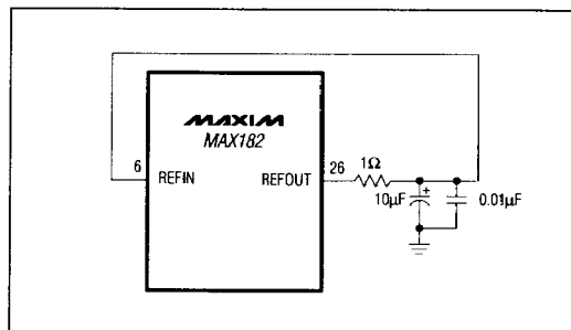
Figure 17. Internal Reference Hookup.
