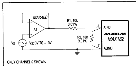
Figure 13. Unipolar 0V to +10V Operation
