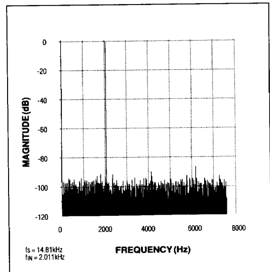
Figure 20. FFT Plot for the MAX182
