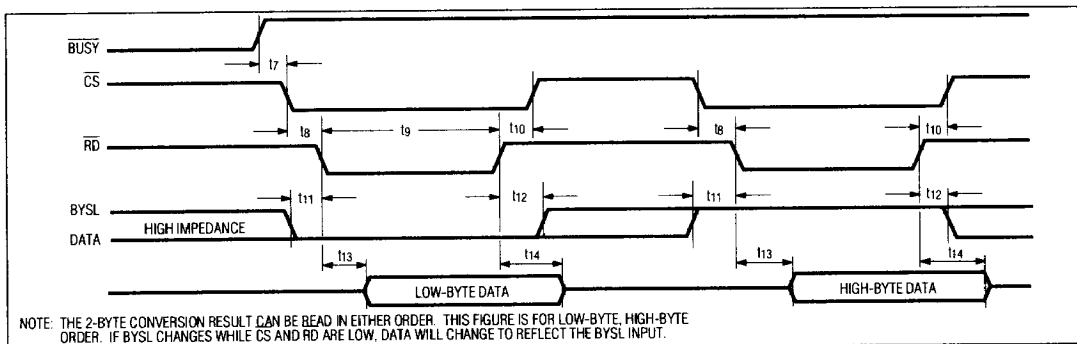
Figure 2. Read Cycle Timing
