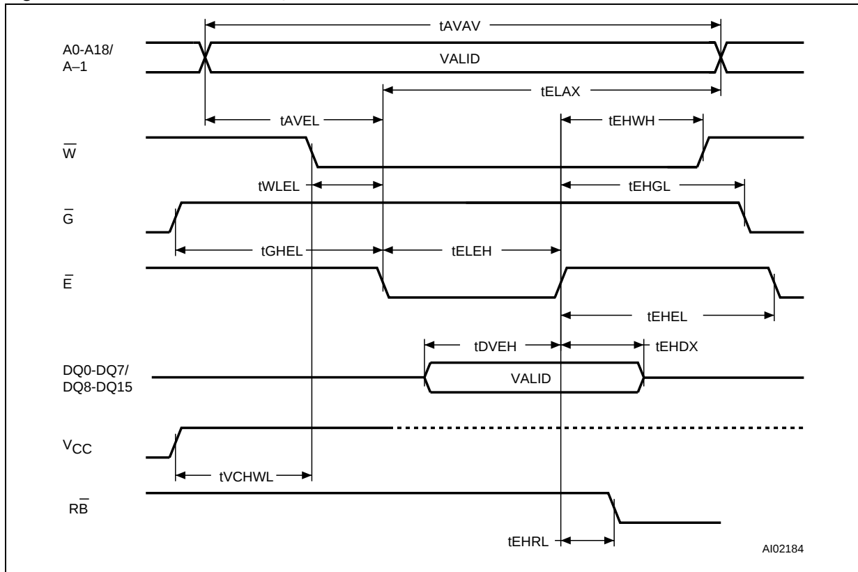
Figure 10. Write AC Waveforms, \overline{E} Controlled
