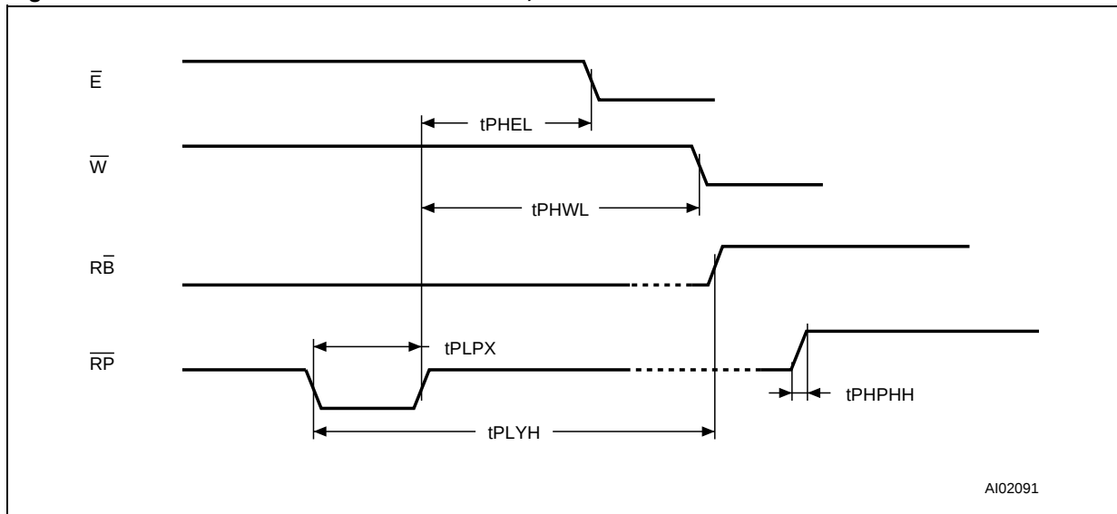
Figure 11. Read and Write AC Characteristics, \overline{RP} Related
