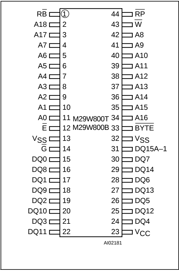
Figure 4. SO Connections
